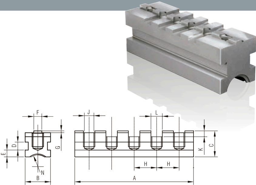
GARRA PARTIDA BASE HARD MASTER JAW
